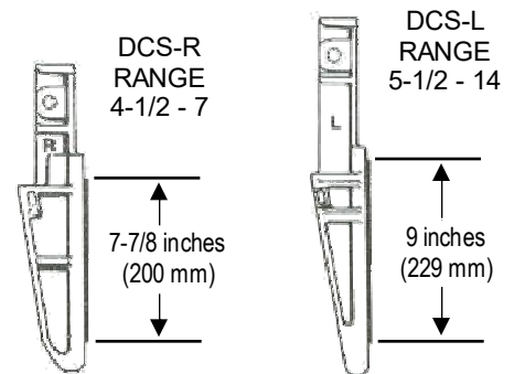
DCS Slip Grip Lengths
