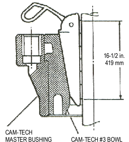
CAM-TECH SDXL ROTARY SLIPS
