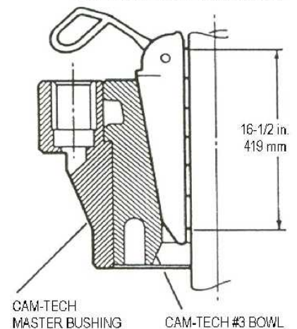
CAM-TECH SDXL ROTARY SLIPS
